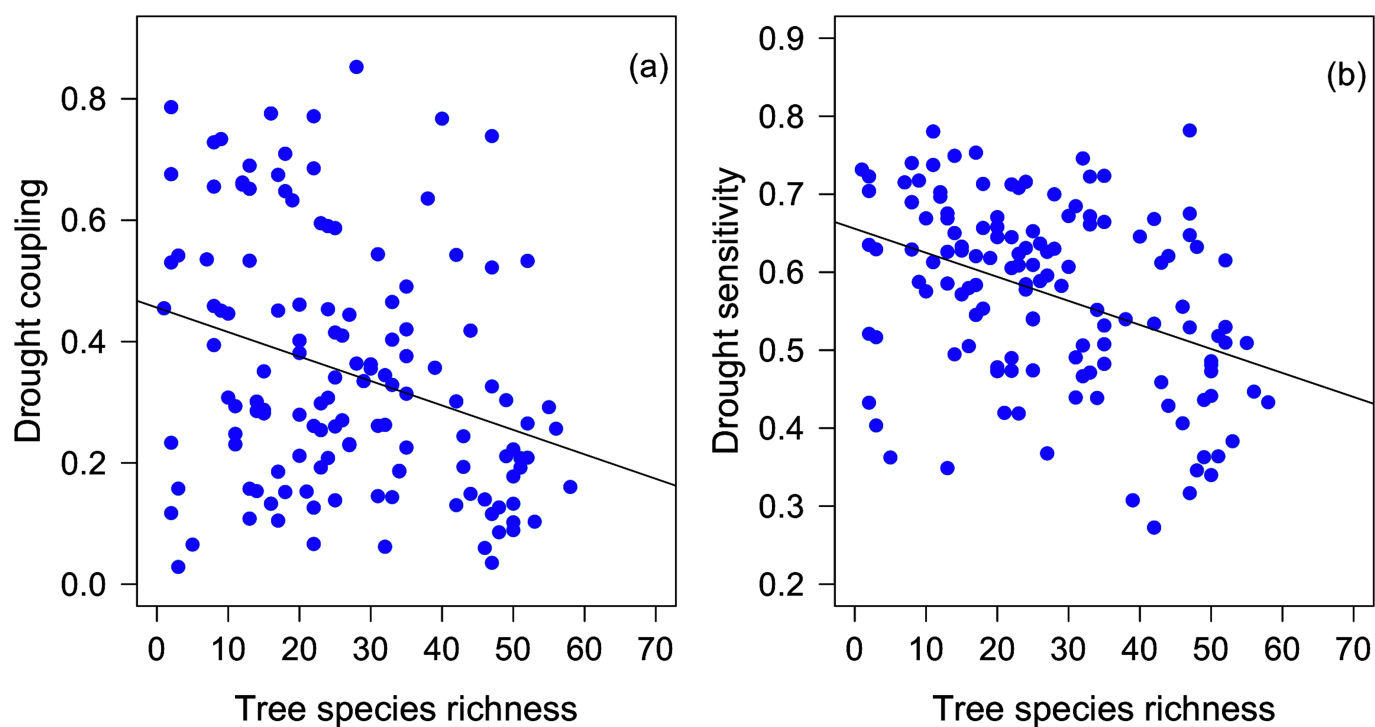
Extended Data Fig. 6 | Higher species diversity is associated with more buffered drought responses in US forests. a, b, Drought coupling (a; n = 163 grid cells) and drought sensitivity (b; n = 163 grid cells) from
