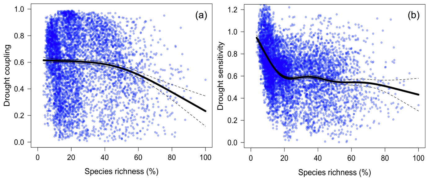
Extended Data Fig. 9 | Ecosystem sensitivity to drought saturates with species richness (the percentage of maximum) across forests globally. a , Drought coupling is expressed as the explained variation ( R^2 ) of midday aboveground plant water content in forest ecosystems regressed against drought variables using ordinary least-squares linear regression.
