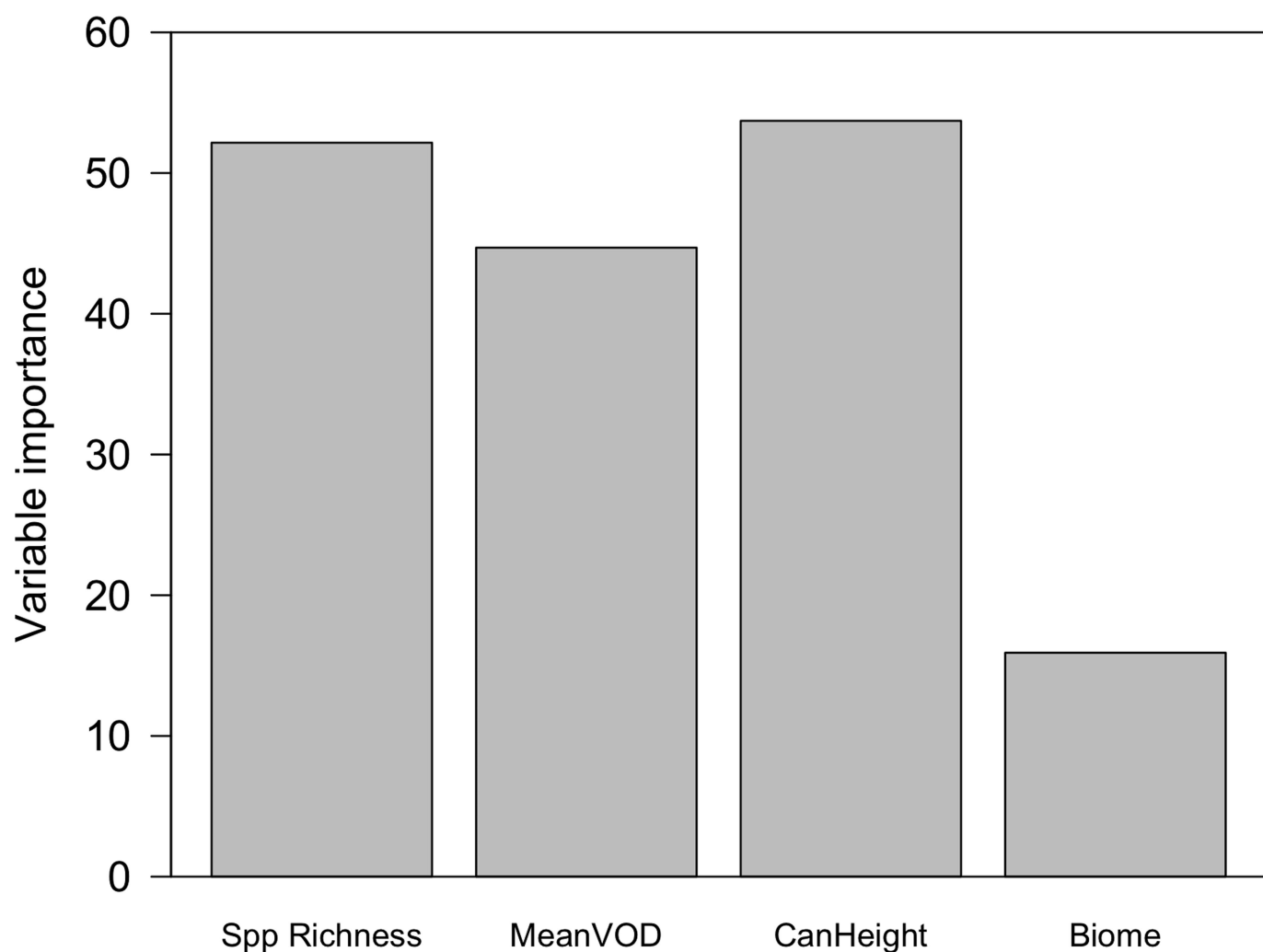
Extended Data Fig. 8 | Analyses of the importance of variables using satellite data. The importance of the variables (total decrease in node impurities) results obtained using the machine learning algorithm,
