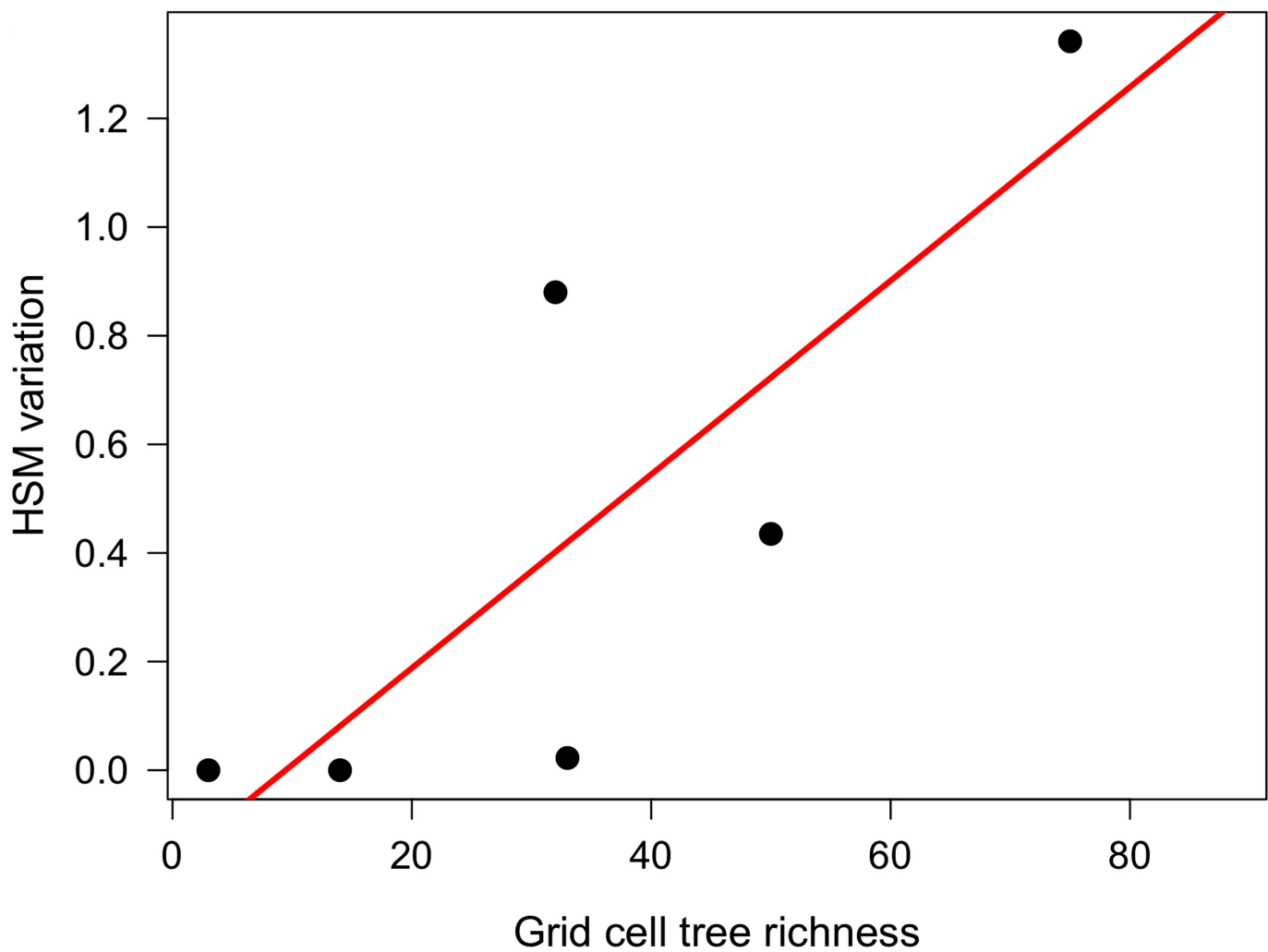
Extended Data Fig. 5 | Hydraulic trait variation compared to species richness. Comparison of dominant tree species richness from gridded data of US forests against the hydraulic diversity—the standard deviation
